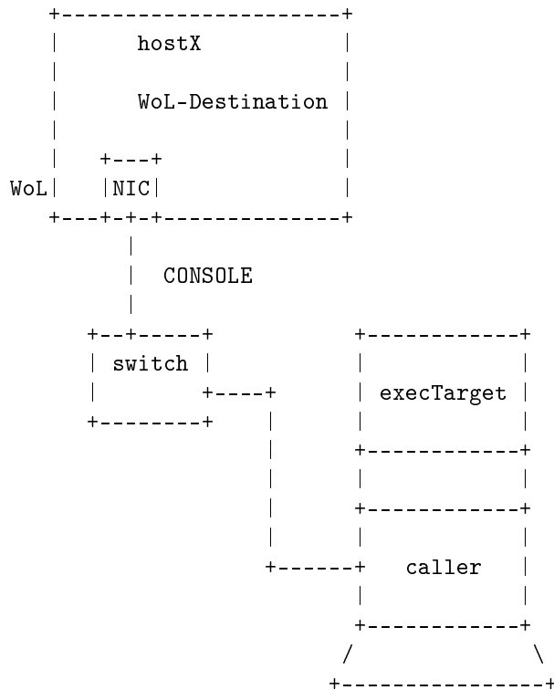
Figure 23.1: "Bridge-less" WoL configuration within same Ethernet Segment
