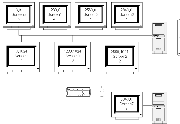
Figure 5.9: Physical Multi-Monitor Layout-2
