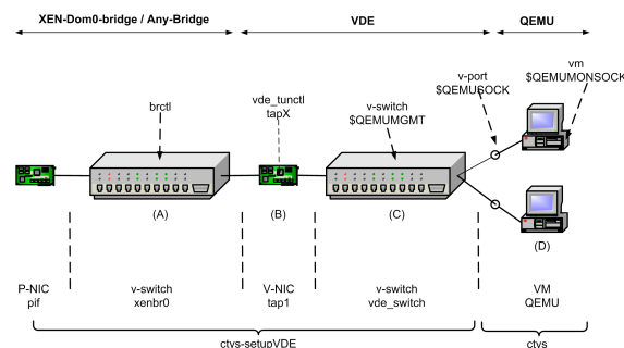
Figure 8.5: QEMU/KVM-Network Interconnection - Details
