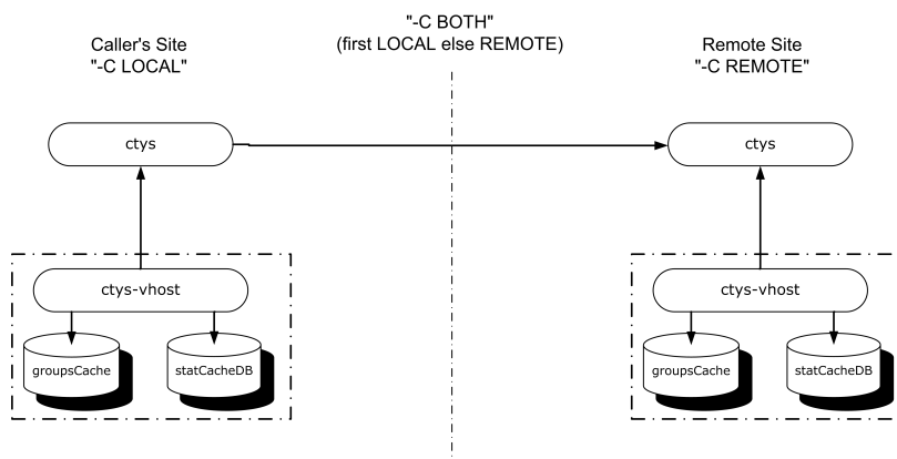
Figure 6.3: Distributed Caches
