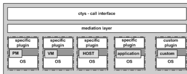
Figure 8.2: ctys SW-Layers and plugins
