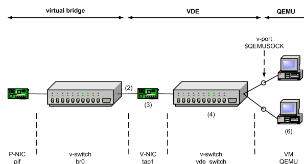
Figure 8.3: QEMU/KVM-Network Interconnection
