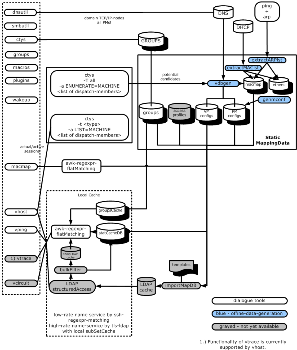
Figure 9.1: Nameservice components
